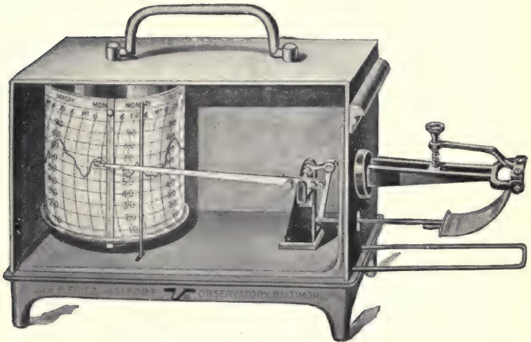
FIGURE 16. Richard's Thermograph.
